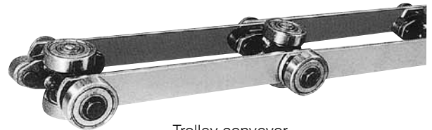
Trolley conveyor
